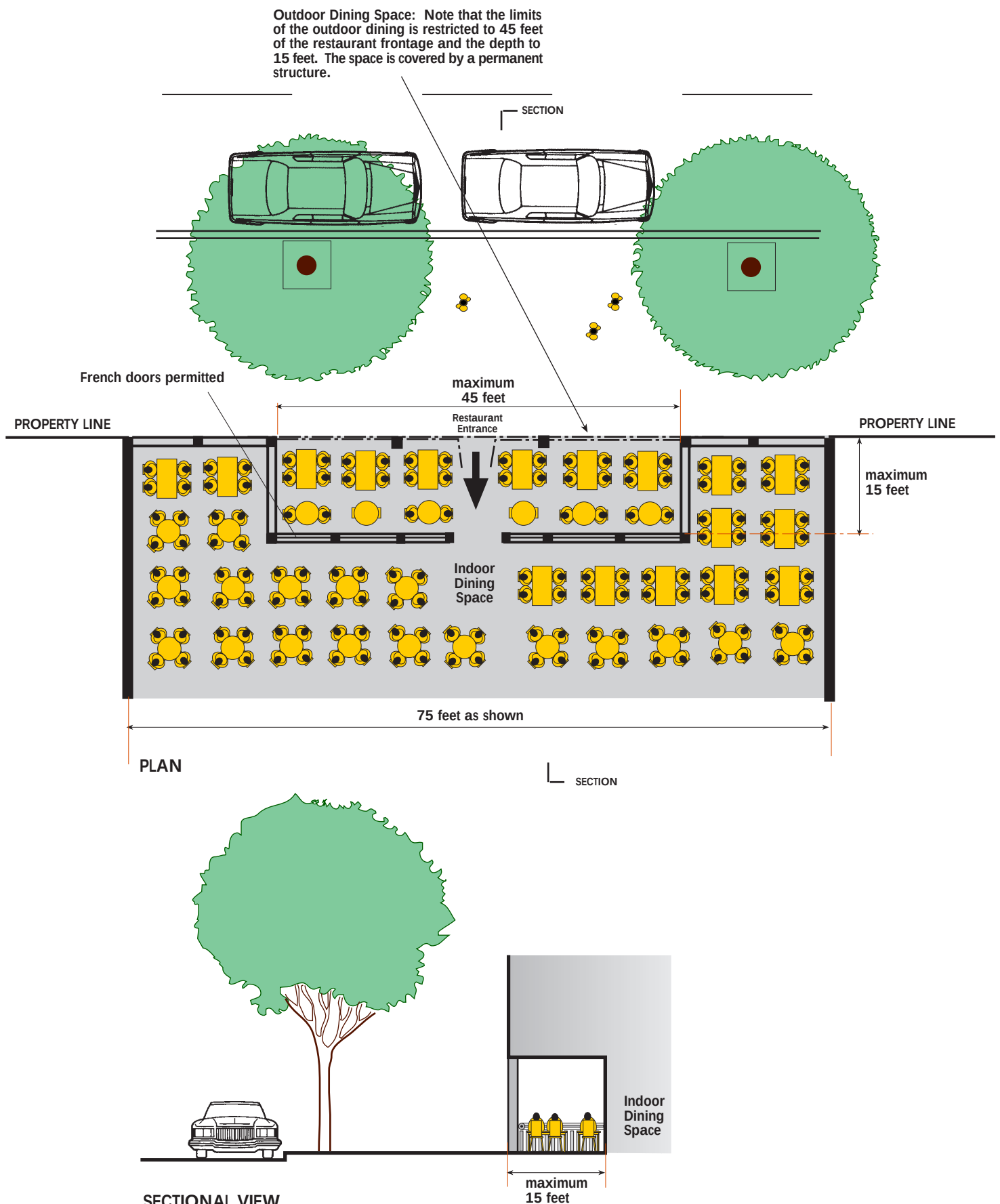
Figure 3.11: Outdoor Dining: Typical Layout (For stores with a frontage greater than 60 feet)
