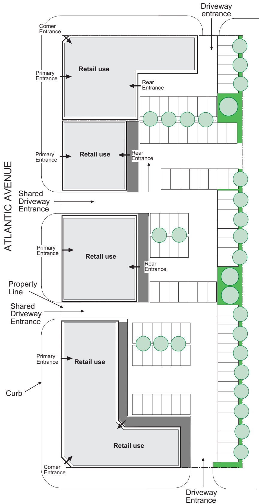
Figure 3.12: Typical block plan: Transition (Mixed-use) Subarea
