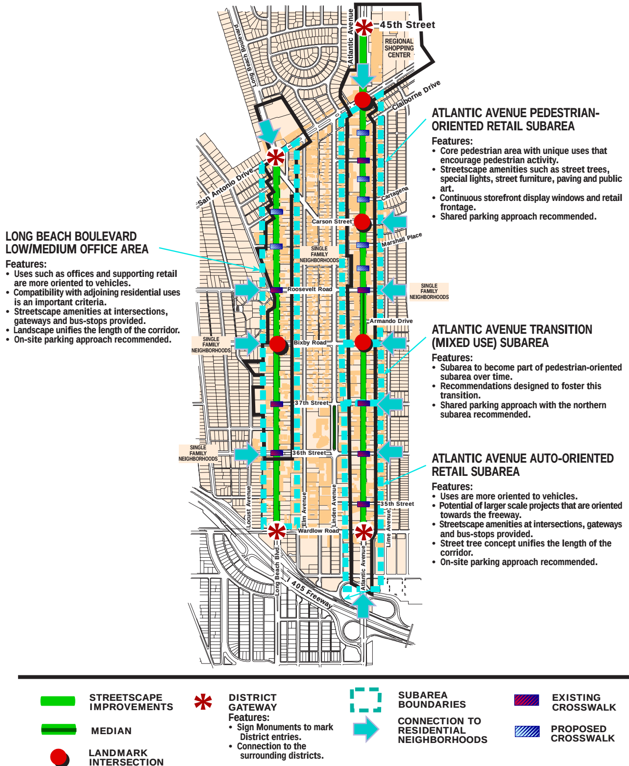
Figure 2.1: Concept Plan
