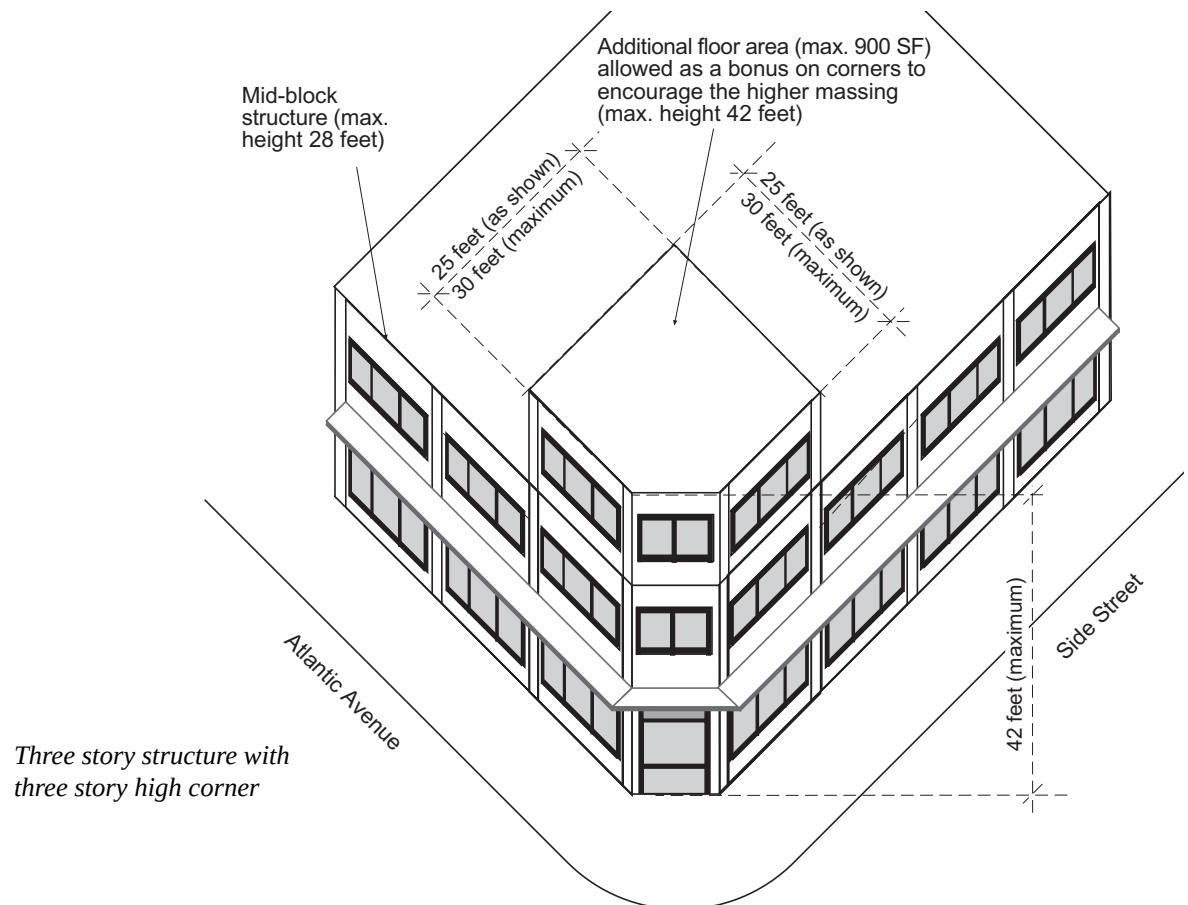
Figure 3.1: Typical corner condition: heights and massing
