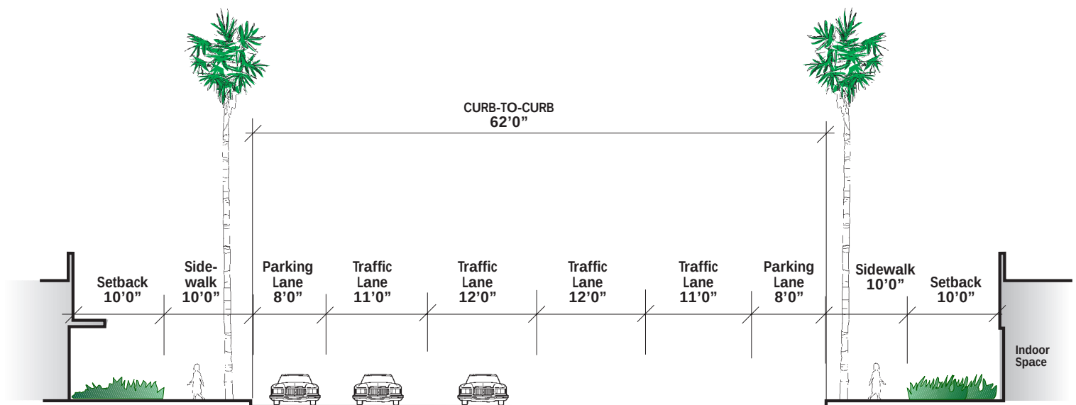
SECTIONAL VIEW (Looking north)
